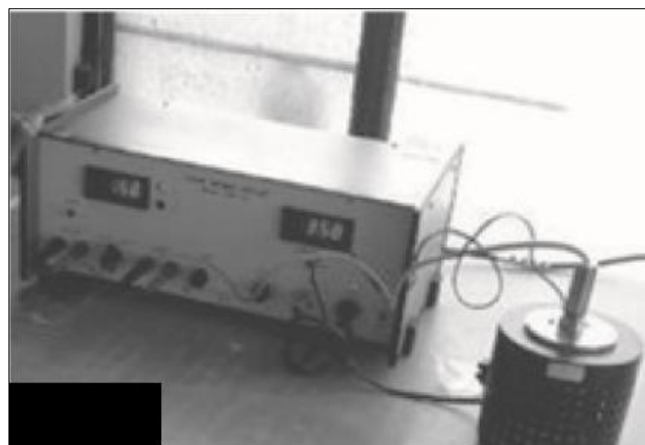
Fig 1: Experimental Set- up of DC Conductivity Measurement
