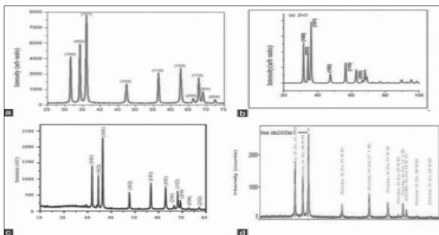
Fig 2: Powder X-ray diffraction (a) with glycine as fuel, (b) with citric acid as fuel, (c) with urea as fuel, and (d) with Raphanus sativus as fuel
