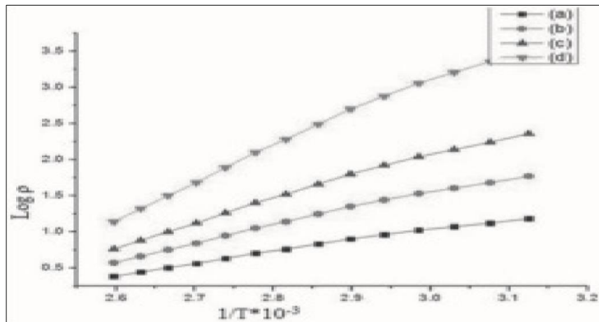
Fig 4: DC Conductivity Studies of Zinc Oxide Nanoparticles (a) with Glycine as Fuel, (b) with Citric Acid as Fuel, (c) with Urea as Fuel, and (d) with Raphanus Sativus as Fuel
