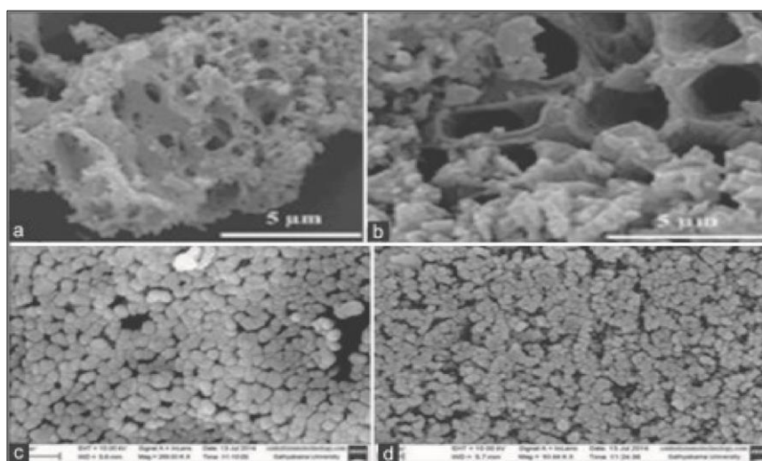
Fig 3: Field emission scanning electron microscopy images of zinc oxide nanoparticles (a) with glycine as fuel (b) with citric acid as fuel (c) with urea as fuel and (d) with Raphanus sativus as fuel.
