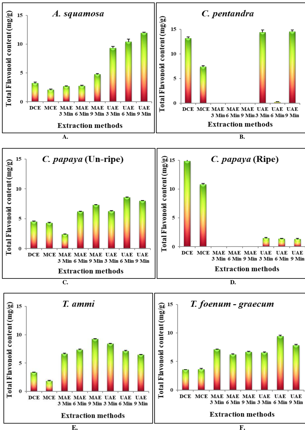
Fig 4: Effect of extraction methods and time on total flavonoid content of some medicinal plant seeds
